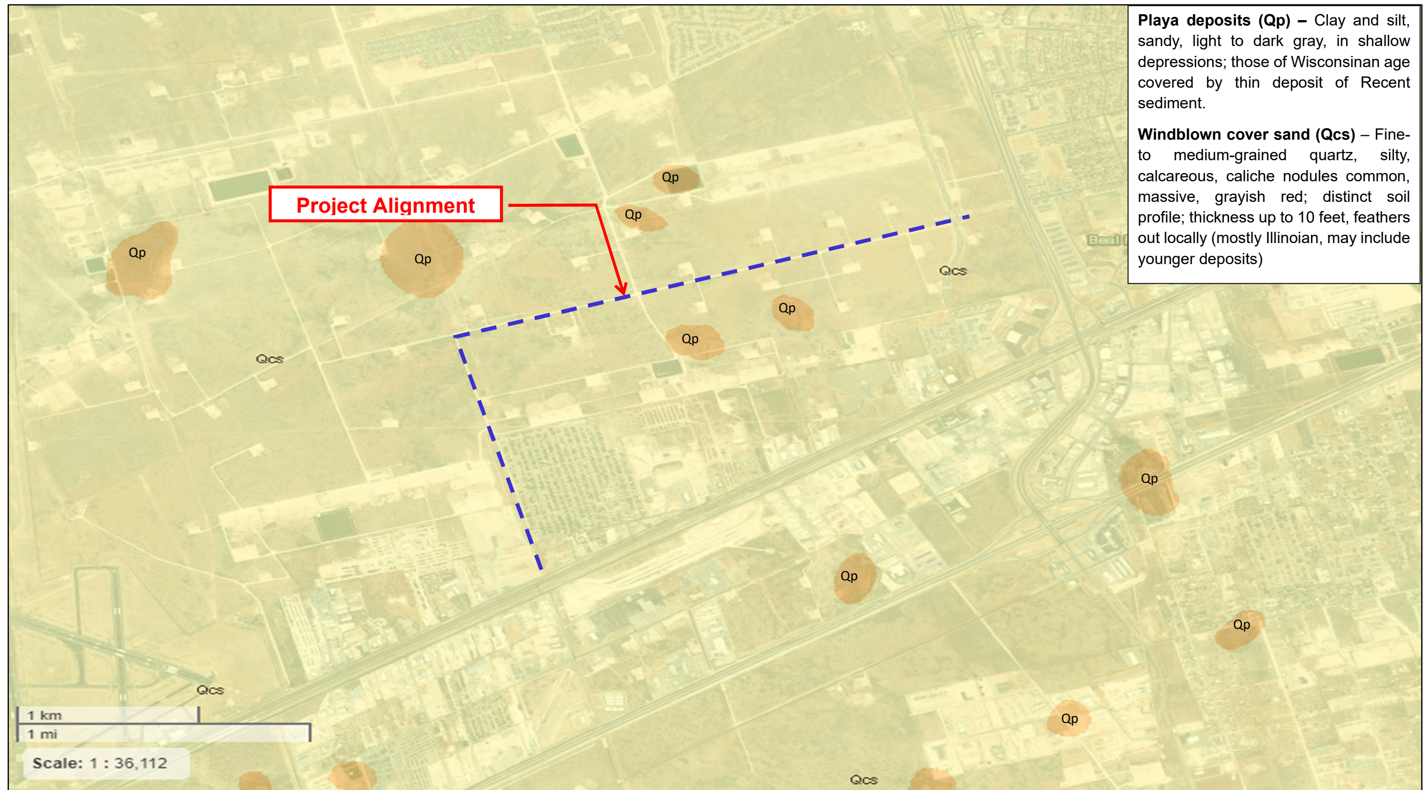
Figure 3 – Site Vicinity Geologic Map
