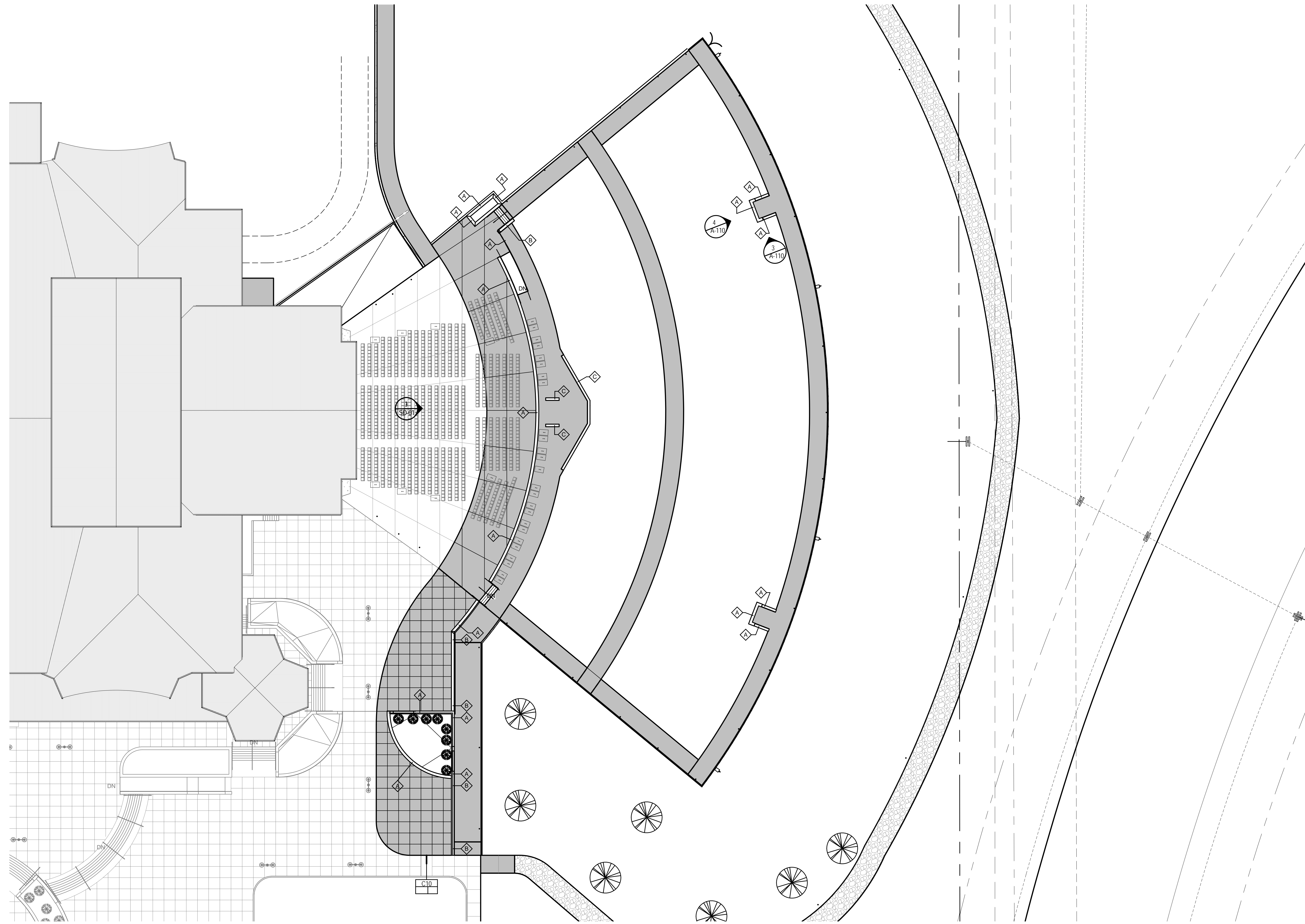
1 SITE PLAN SD-02 1" = 20'-0"
