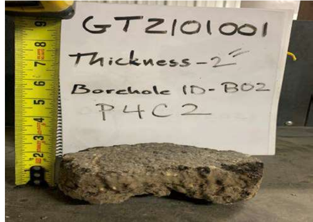
P4C2 B-2 - 2 in Asphalt Core
