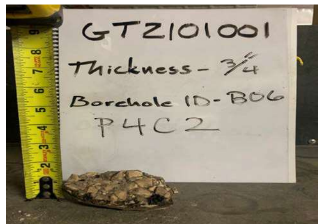
P4C2 B-6 - 3/4 in Asphalt Core
