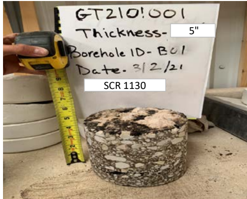
SCR 1130 B-1 - 5 in Asphalt Core
